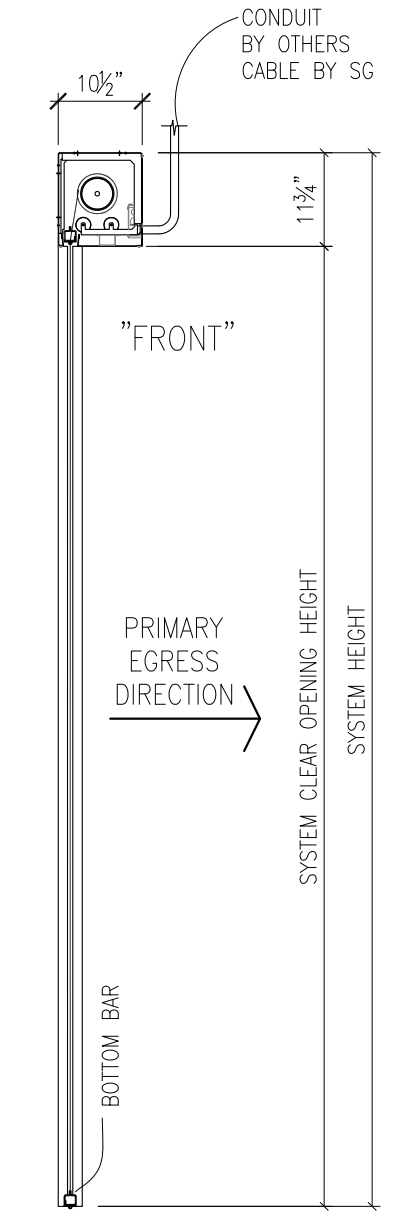
B SECTION
