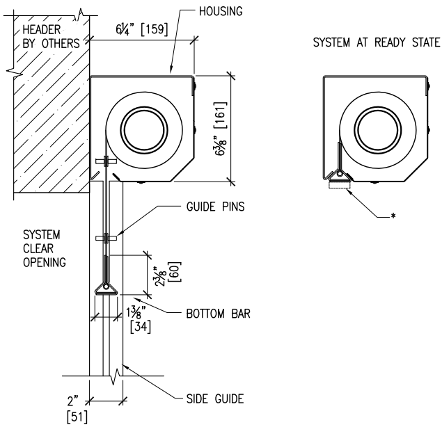
(E) HEAD DETAIL 1 1/2" = 1'-0"
