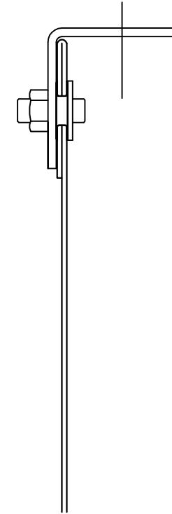
INSTALLATION DETAIL @ UPPER EDGE
