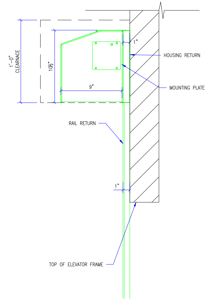
③ M200 HOUSING DETAIL SCALE: 1 1/2" = 1'-0"
