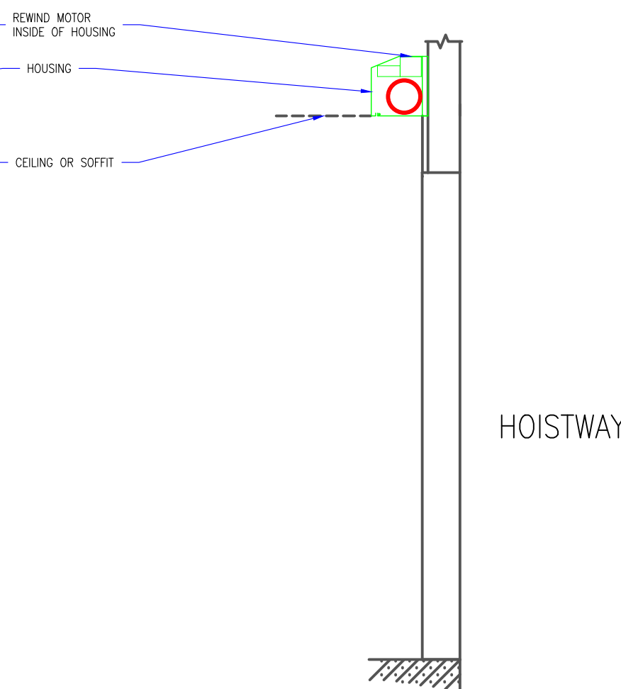
SECTION - READY STATE
