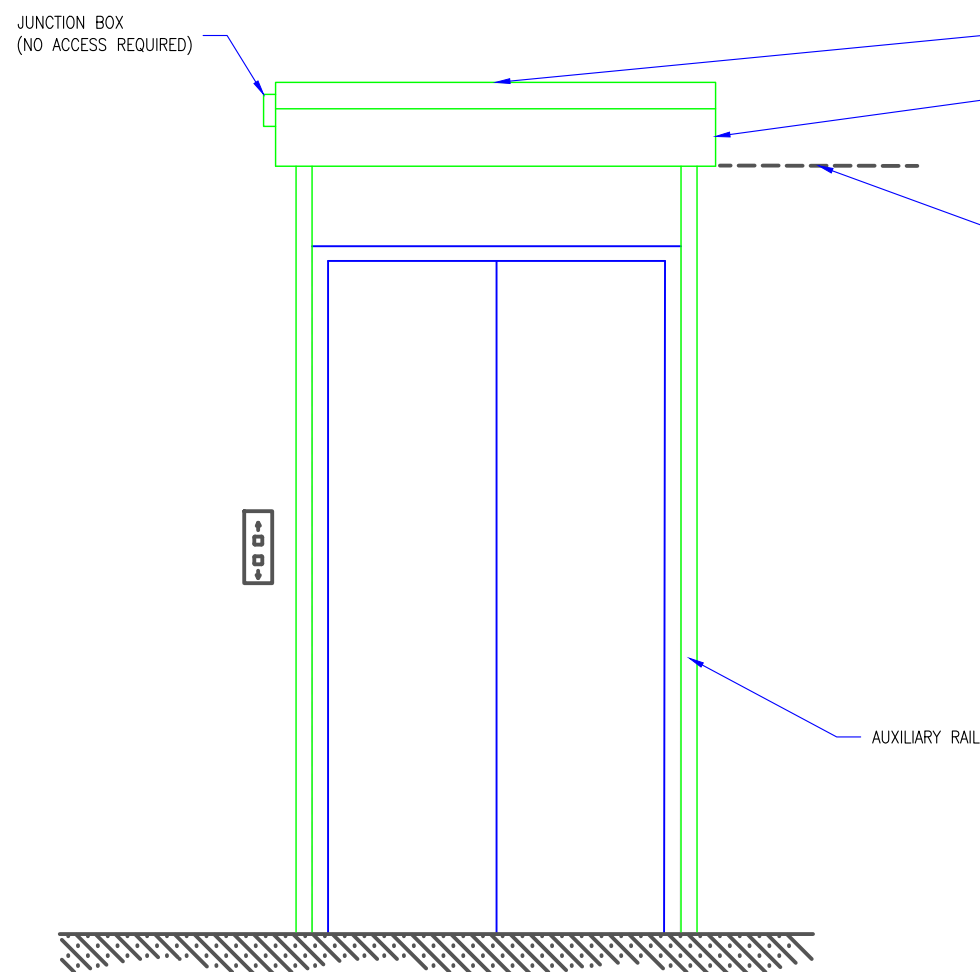
LANDING ELEVATION - READY STATE
