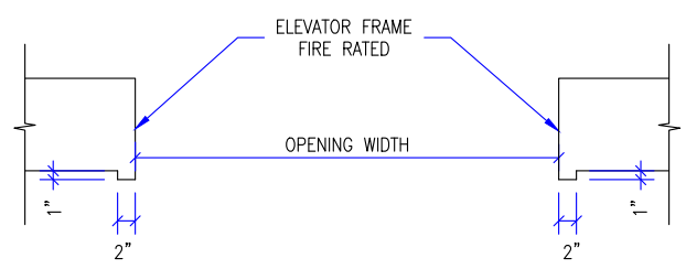
④ M200-JAMB SECTION DETAIL SCALE: 1/2" = 1'-0"
